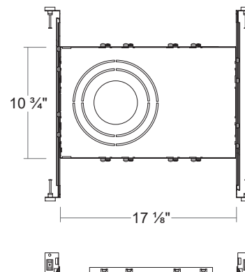
LRPHB-80 Mounting Plate / Round / for 4, 6, 8 inch
