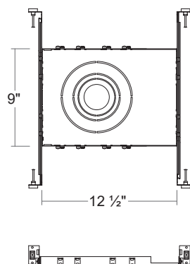
LRPHB-60 Mounting Plate / Round / for 2, 3, 4, 6 inch
