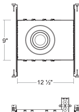
LRPJB-60 Mounting Plate / Round / for 2, 3, 4, 6 inch
