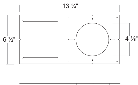
LRP40 4" Mounting Plate / Round
