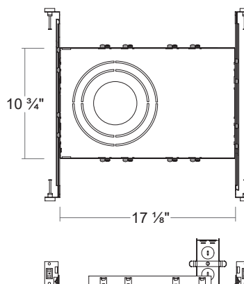
LRPJB-80 Mounting Plate / Round / for 4, 6, 8 inch
